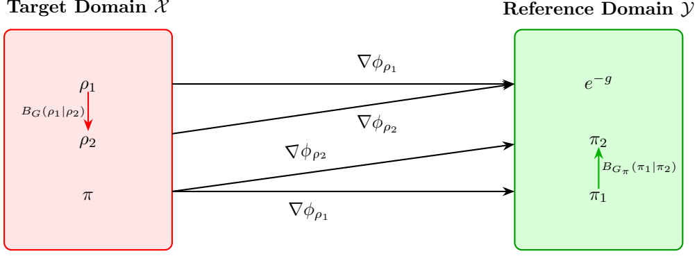
Figure 1: The probability densities \rho_1, \rho_2, \pi live on the target domain \mathcal{X} while the densities \pi_1, \pi_2, e^{-g} live on the reference domain \mathcal{Y} . \nabla\phi_{\rho_i} is the Brenier map from \rho_i to e^{-g} , i = 1, 2 . As \pi_i = \nabla\phi_{\rho_i} \# \pi , Brenier’s Theorem [Bre91] implies that \nabla\phi_{\rho_i} is also the Brenier map from \pi to \pi_i , for i = 1, 2 . The telescoping term in Lemma 3.1, B_G(\pi|\rho_1) - B_G(\pi|\rho_2) involves densities \rho_1, \rho_2, \pi all of which live on the target space. One might naturally expect the transportation cost to be B_G(\rho_1|\rho_2) . In sharp contrast, the corresponding term in Lemma 3.1 is B_{G_\pi}(\pi_1|\pi_2) where \pi_i lives on the reference domain and is the image of \pi under the Brenier map \nabla\phi_{\rho_i} , i = 1, 2 .
