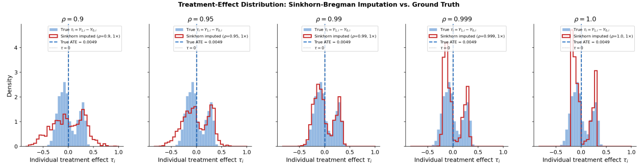
(c) Imputed TED \mathcal{L}_\rho(\widehat{Y}_1 - Y_0) , Bregman-Sinkhorn copula DGP, varying \rho .
